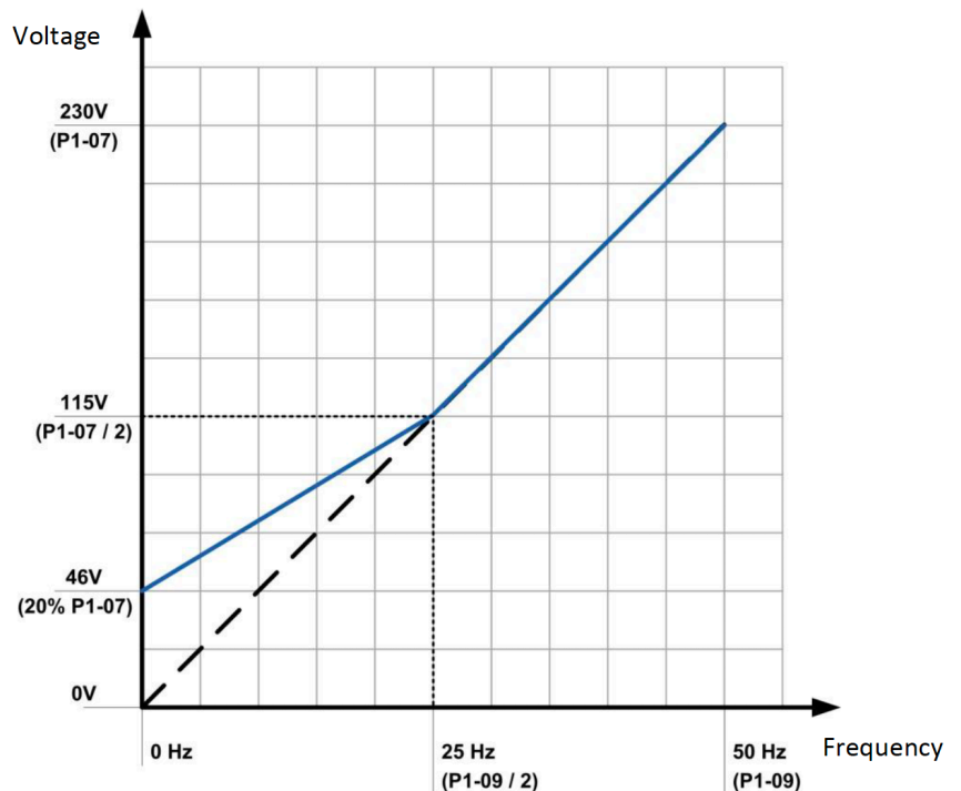
--- Normal V/F Characteristic — Boost Adjusted V/F Characteristic
