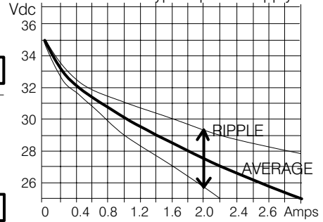
Performance of typical power supply
